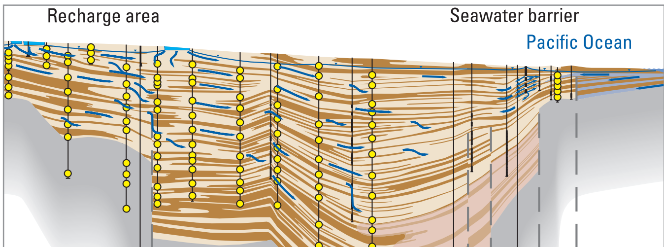
Groundwater monitoring improves insight into groundwater flow within the OCWD service area in Southern California.
